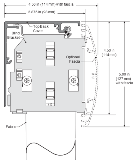
Installed Profile: 3 inch Blind (Fascia end caps and some other details omitted for clarity.)
