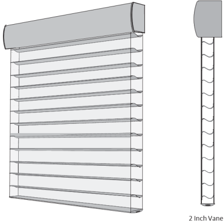
Installed Profile: 2 inch Blind (Fascia end caps and some other details omitted for clarity.)
