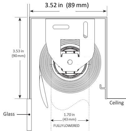
Installed Profile: 3 inch Blind (Fascia end caps and some other details omitted for clarity.)
